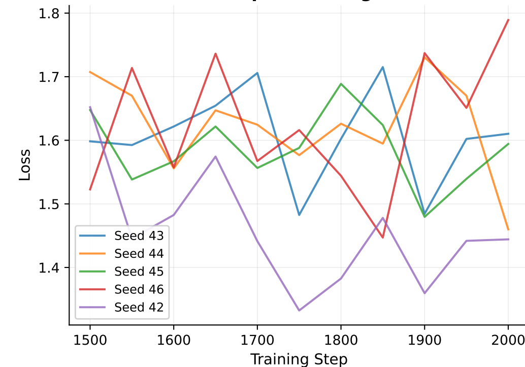
Post-Collapse Training Curves
