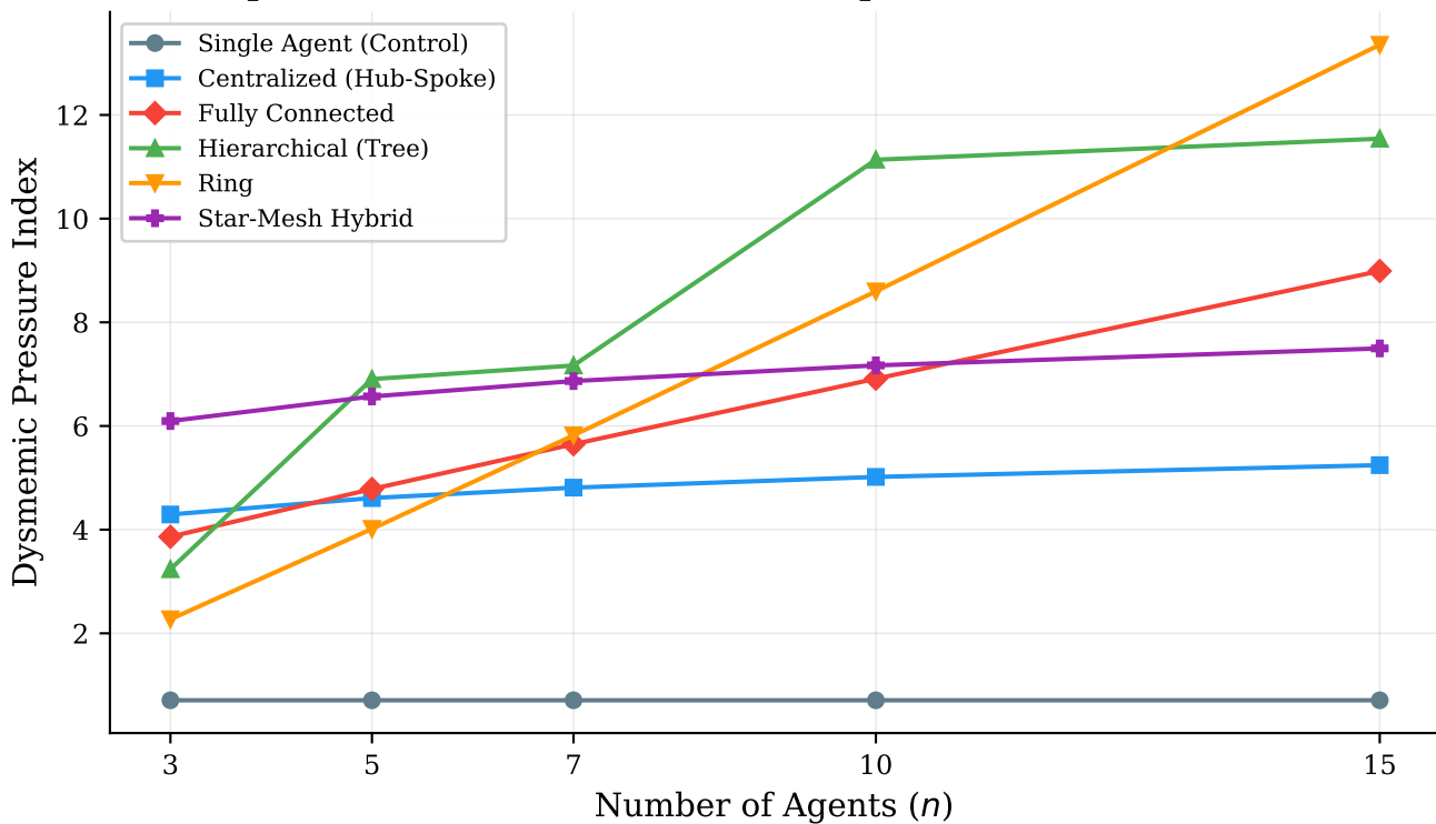
Dysmemic Pressure Index by Architecture (Compound information loss from compression, selection, and drift)
