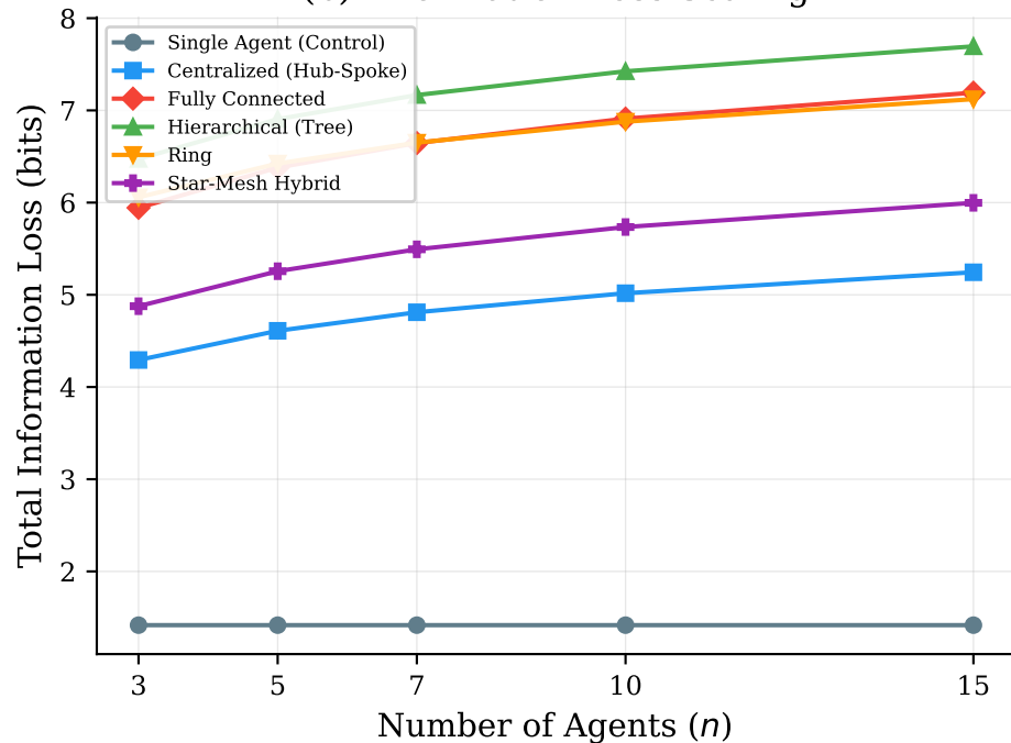
(b) Information Loss Scaling
