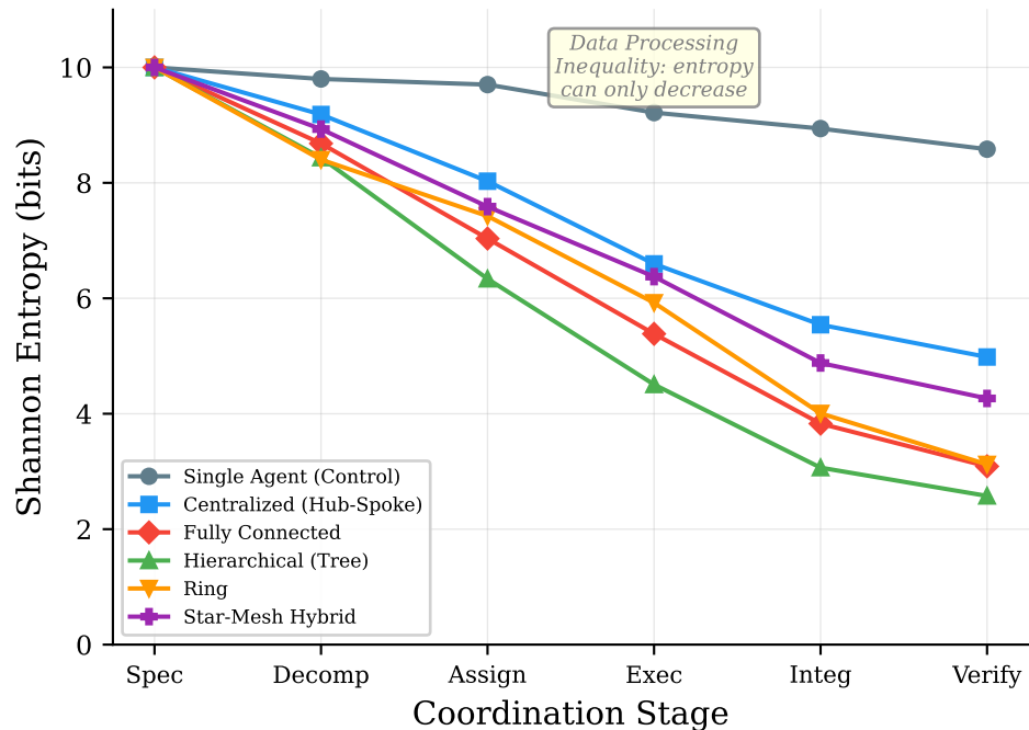
(a) Information Preservation at n = 10
