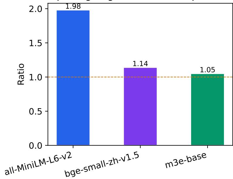
Discrimination Ratio (top / avg, higher = better separation)
