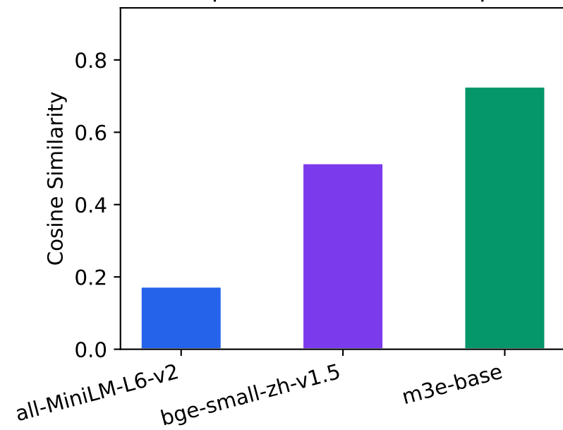
Avg Cosine Similarity (model-specific, not cross-comparable)
