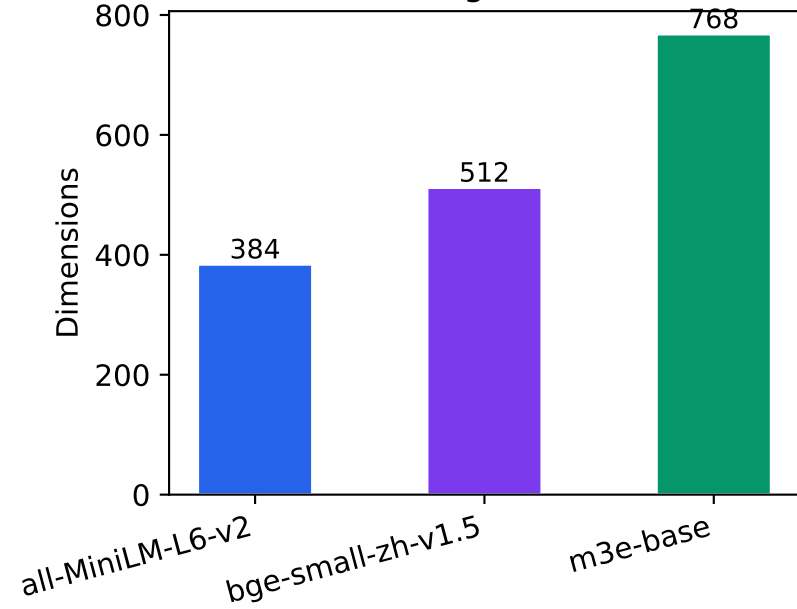
Embedding Dimension
