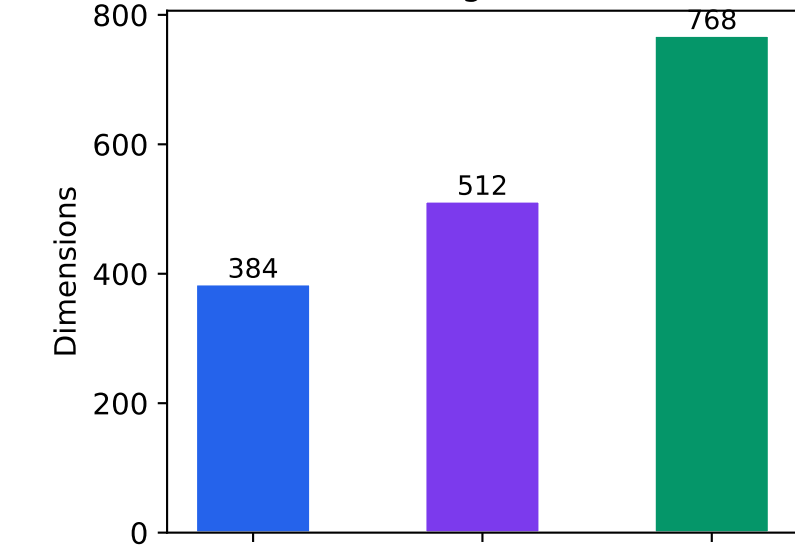
Embedding Dimension
