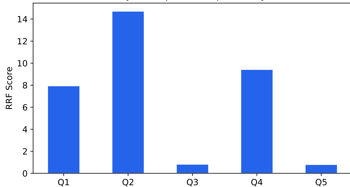
Hybrid Top-1 Score per Query
