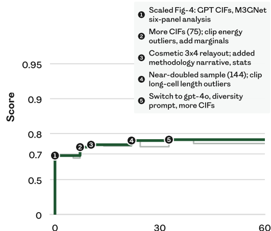
Foundational Large Language Models for Materials Research: Figure 4
