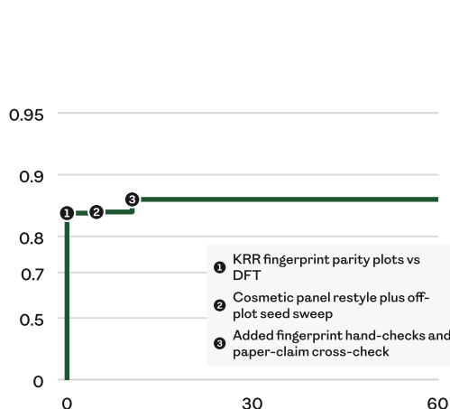
Accelerating Materials Property Predictions Using Machine Learning: Figure 2
