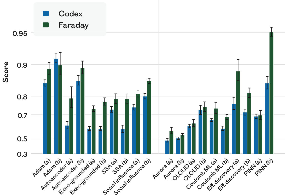
ML (train)
