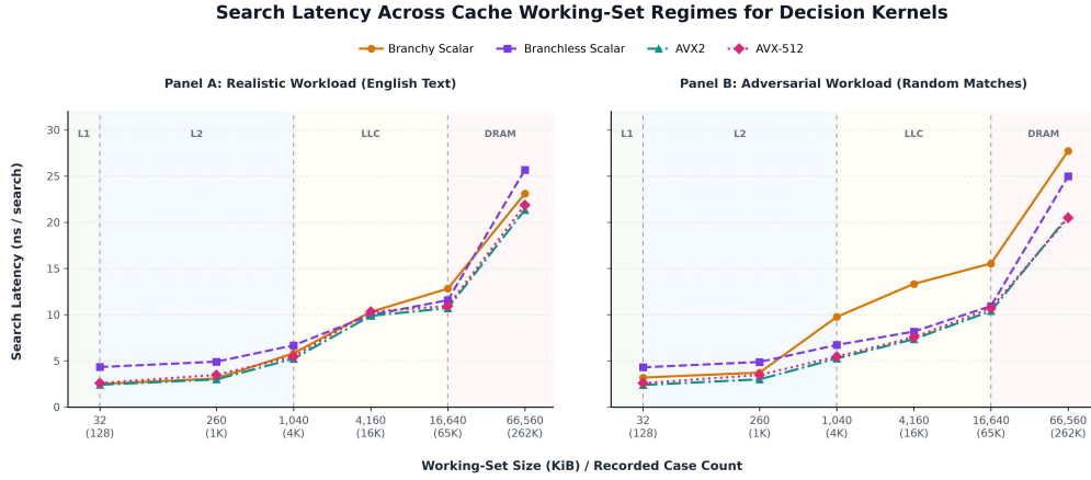
Figure 4: Search latency (ns / search) of decision kernels across hardware cache residency regimes (L1, L2, LLC, and DRAM) for predictable English text (Panel A) and branch-unpredictable adversarial workloads (Panel B). On predictable text, the branchy scalar kernel achieves low latency in L1 due to accurate branch prediction. Under adversarial conditions, branchy scalar latency degrades sharply in the L2 and LLC regimes owing to branch misprediction penalties. Vectorized SIMD kernels (AVX2 and AVX-512) eliminate branch mispredictions and consistently maintain minimal latency across compute-bound cache regimes, converging with other implementations as memory bandwidth limits performance in DRAM.
