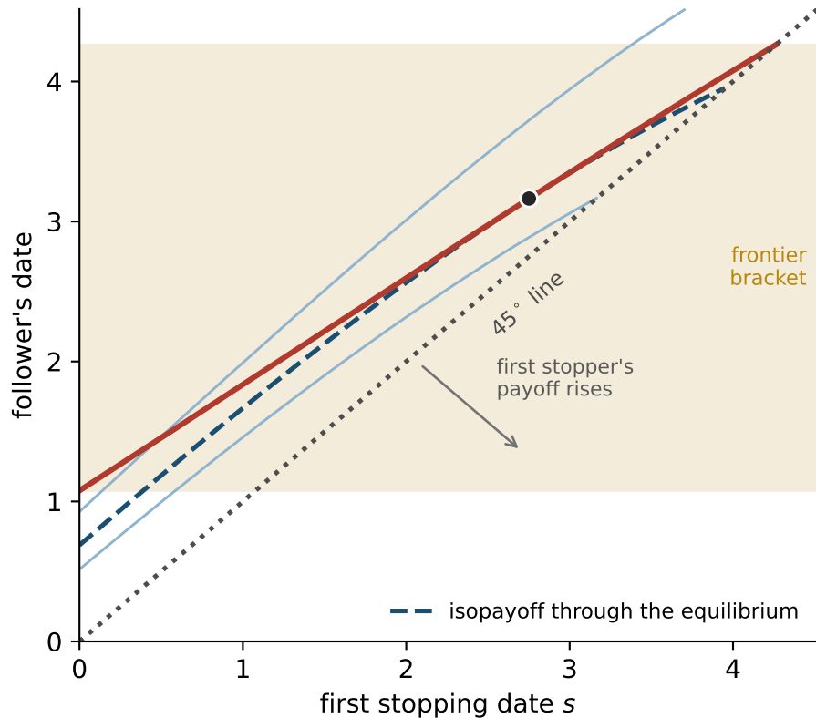
(b) score contest, \gamma = 2 : interior tangency
