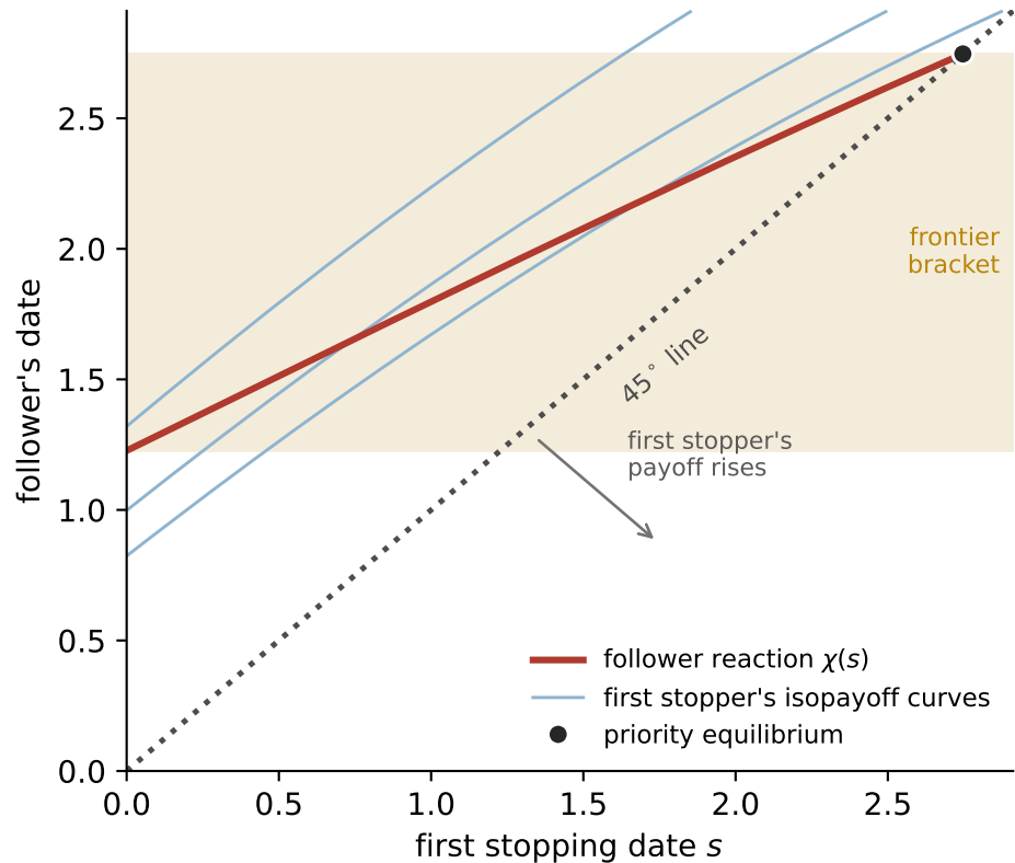
(a) score contest, \gamma = 1 : corner at (\tau^R, \tau^R)
