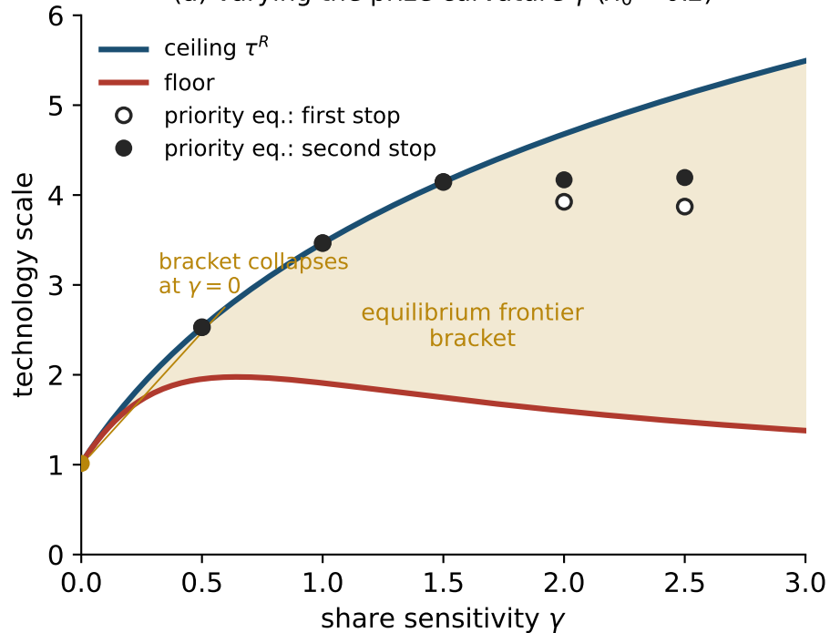
(a) varying the prize curvature \gamma ( \lambda_0 = 0.2 )
