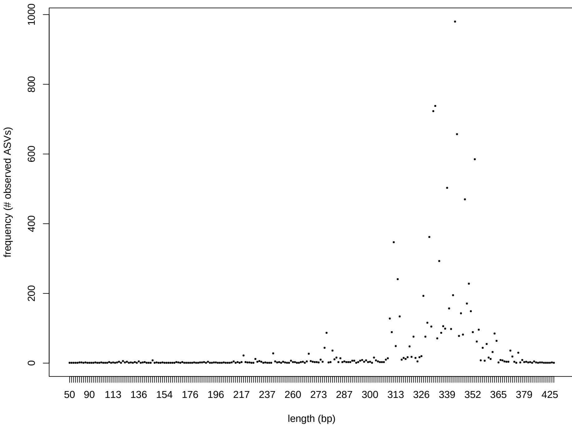
ASV Length Histogram
