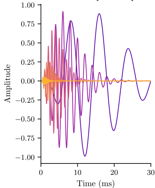
Gammatone impulse responses
