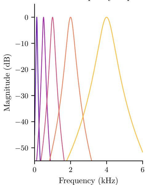
Gammatone frequency responses
