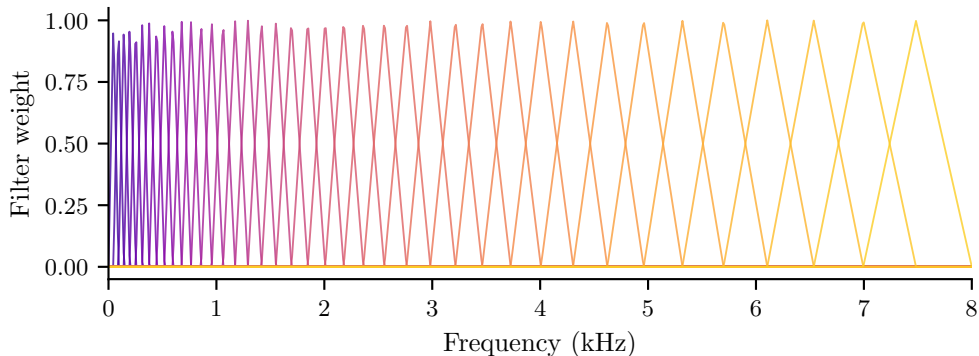
Mel triangular filterbank ( M=40 filters, f_{\min}=0 Hz, f_{\max}=8 kHz)
