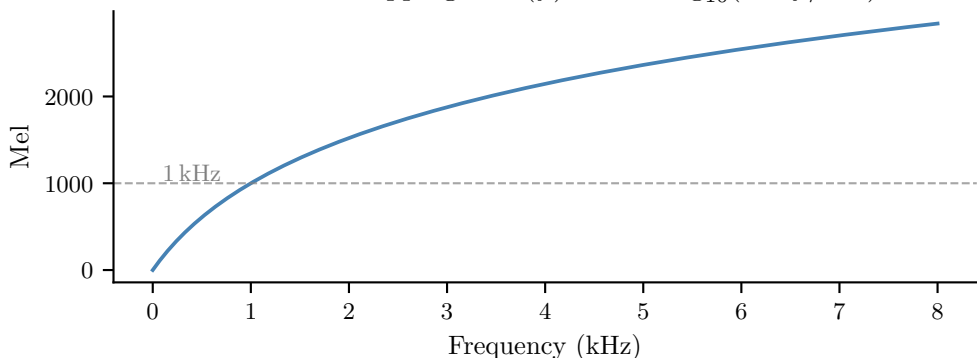
Hz-to-mel mapping: \text{mel}(f) = 2595 \log_{10}(1 + f/700)
