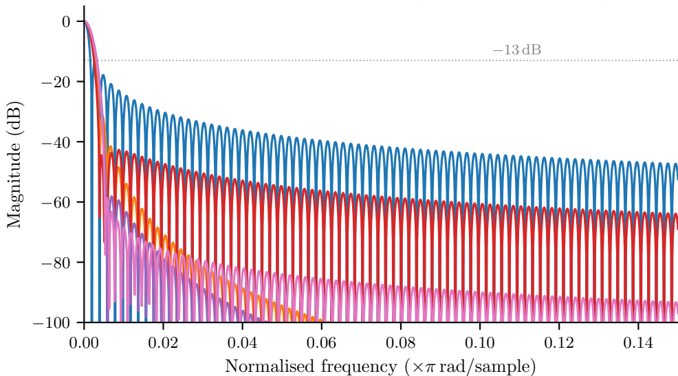
Window frequency responses (zero-padded, N=512 )
