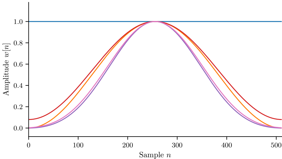
Window functions — time domain ( N = 512 )
