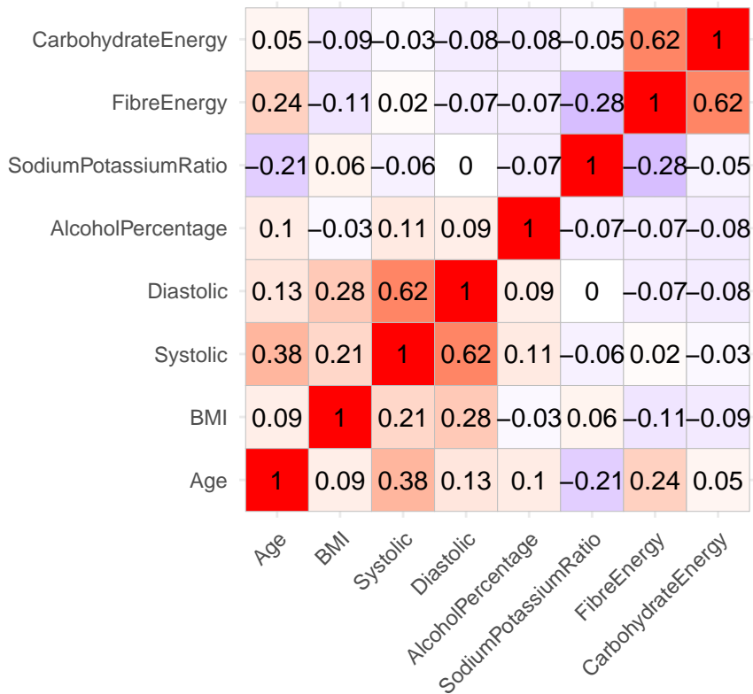
Figure 2: Correlation Heatmap for ALL
