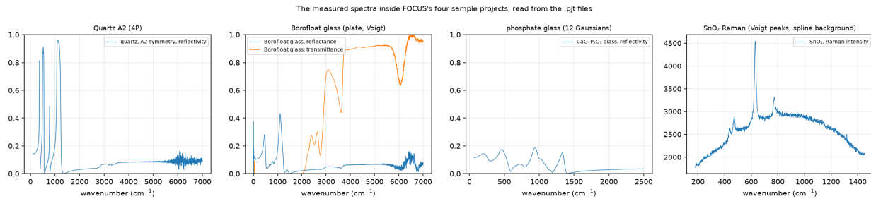
Figure 9: The measured spectra read from the four .pjt files.
