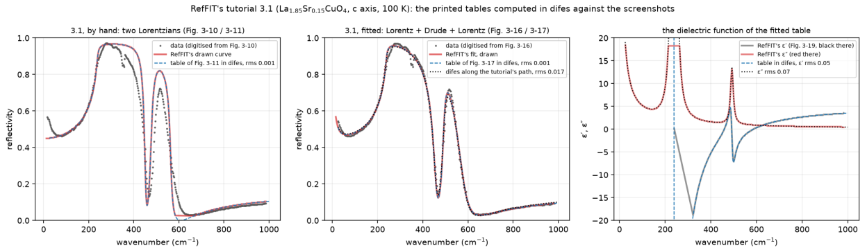
Figure 28: RefFIT’s tutorial 3.1 digitised: the hand model and its curve (left), the fitted model, RefFIT’s curve and difes’s fit along the tutorial’s path (middle), and the fitted table’s \epsilon' and \epsilon'' against RefFIT’s Figure 3-19 (right).
