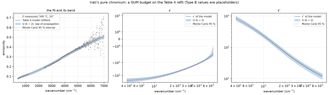
Figure 24: Irati’s pure chromium: the refitted Table 4 model with its expanded-uncertainty band and Monte Carlo interval, and the bands on \varepsilon' and \varepsilon'' , from a budget with placeholder Type B values.
