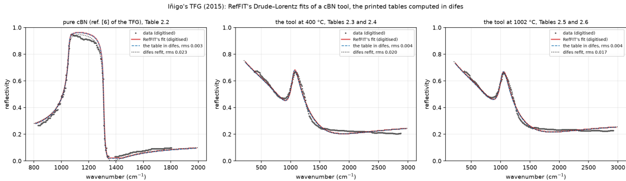
Figure 27: The three figures of the TFG digitised: the data, RefFIT’s fit, the printed table computed in difes and difes’s refit, for pure cBN and for the tool at 400 and 1002 °C.
