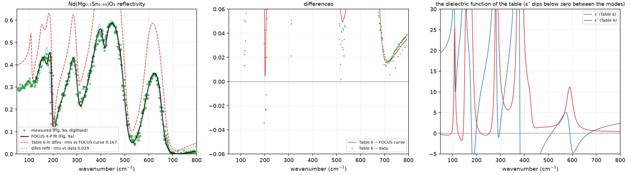
Figure 19: Paper 16: the digitised data and FOCUS curve, Table 6 in difes (dashed), difes's refit (dotted); the table's dielectric function with \varepsilon'' dips below zero between 50 and 253 \text{cm}^{-1} .
