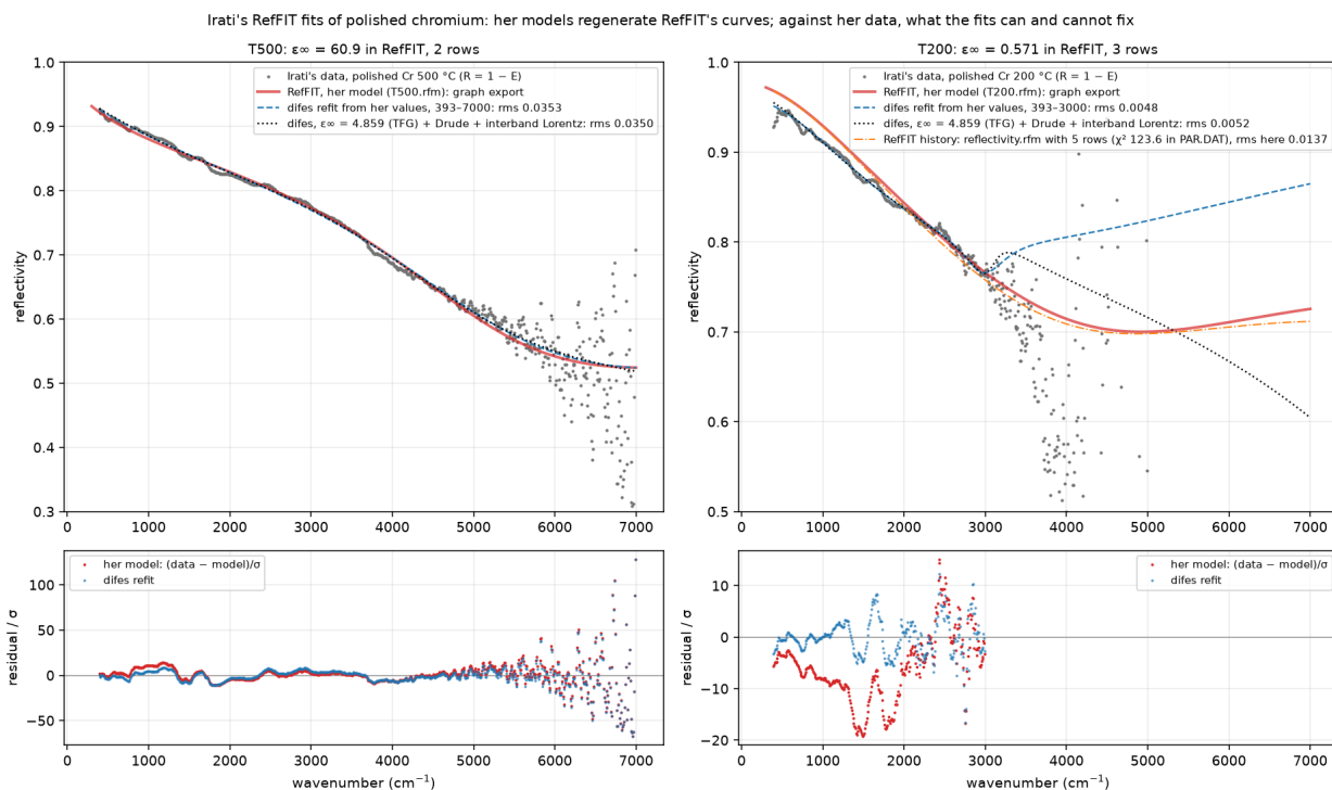
Figure 30: Irati's data (grey), RefFIT's curve of her saved model (red), difes's refit from her values (blue) and the alternative with \epsilon_{\infty} = 4.859 and an interband oscillator (black); below, the residuals in units of her \sigma .
