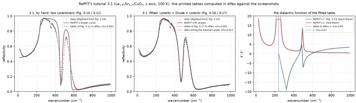
Figure 29: RefFIT's tutorial 3.1 digitised: the hand model and its curve (left), the fitted model, RefFIT's curve and difes's fit along the tutorial's path (middle), and the fitted table's \varepsilon' and \varepsilon'' against RefFIT's Figure 3-19 (right).
