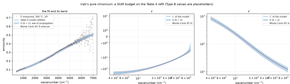
Figure 25: Irati's pure chromium: the refitted Table 4 model with its expanded-uncertainty band and Monte Carlo interval, and the bands on \epsilon' and \epsilon'' , from a budget with placeholder Type B values.
