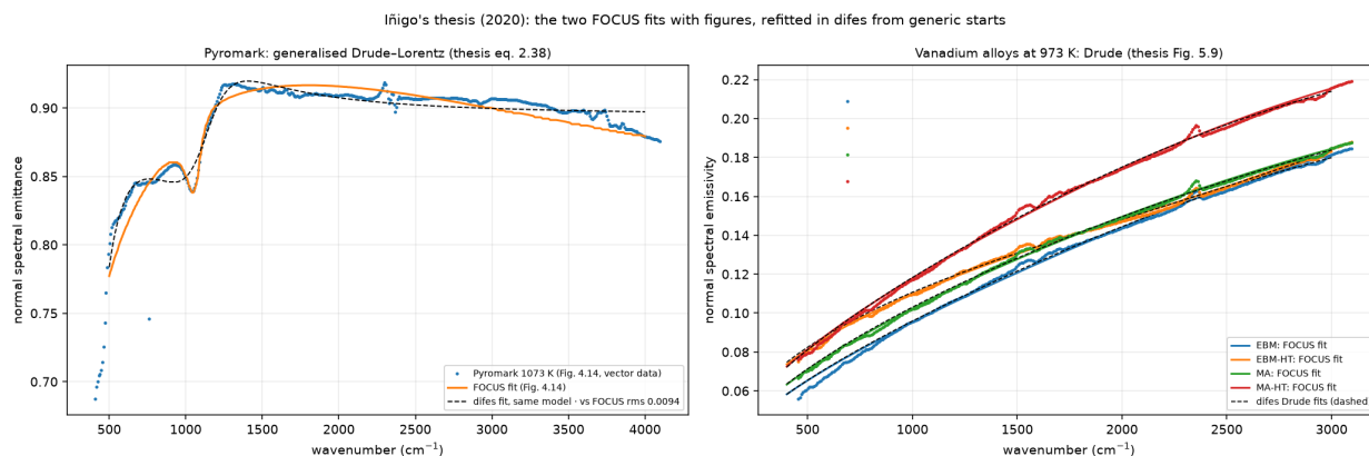
Figure 22: Left: Pyromark at 1073 K, the measured points and FOCUS's fit from Fig. 4.14, and difes's fit of the same model (dashed). Right: Vanadium alloys at 973 K, the measured points and FOCUS's fit from Fig. 5.9, and difes's fit of the same model (dashed).
