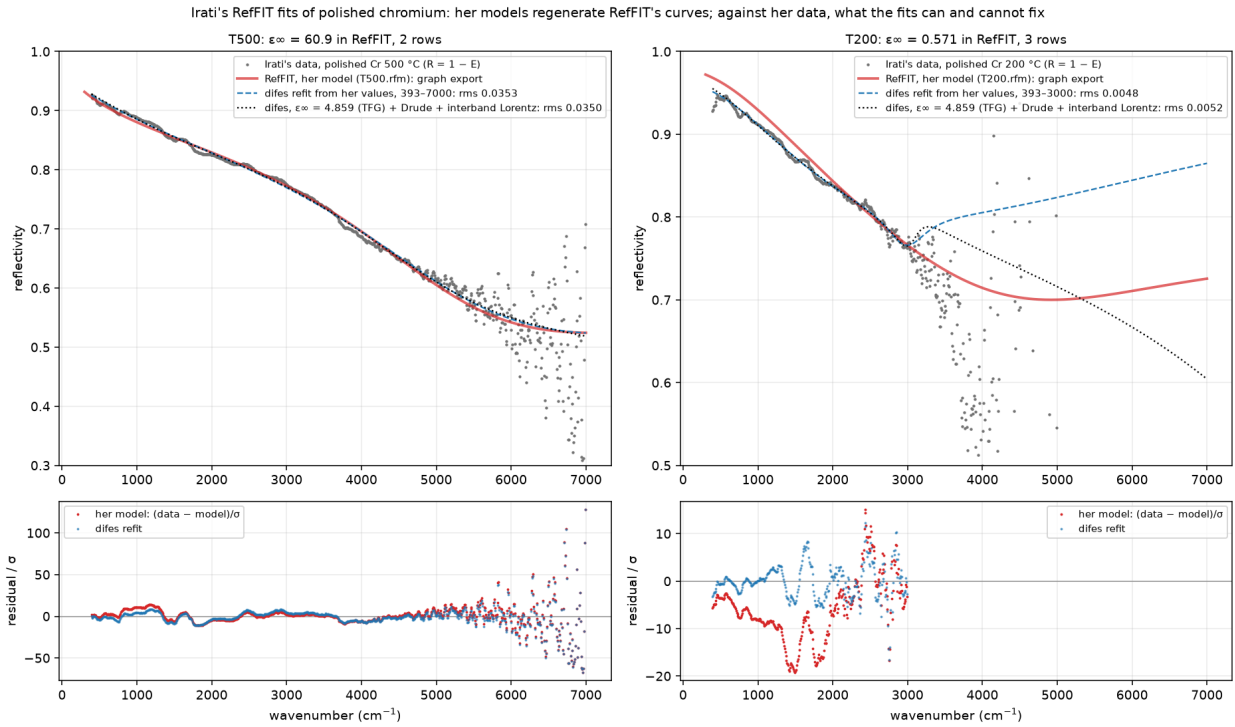
Figure 30: Irati's data (grey), RefFIT's curve of her saved model (red), difes's refit from her values (blue) and the alternative with \epsilon_\infty = 4.859 and an interband oscillator (black); below, the residuals in units of her \sigma .
