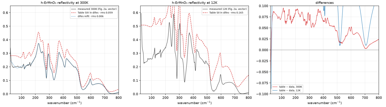
Figure 18: 300 K and 12 K: the vector data, the printed tables in difes (dashed), difes’s refit (dotted); right, table minus data.
