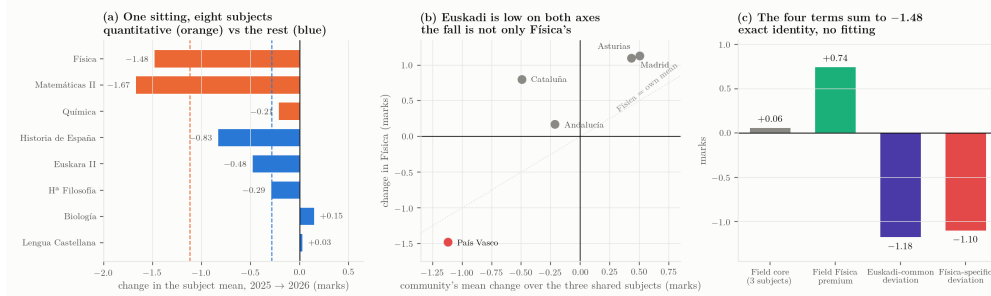
Figure 2: a — the eight Basque subjects, with the three the numerical marking deductions can reach in orange. b — each community's Física change against its own mean over the three shared subjects. c — the four terms of the split, which sum to the observed -1.48 by construction.
