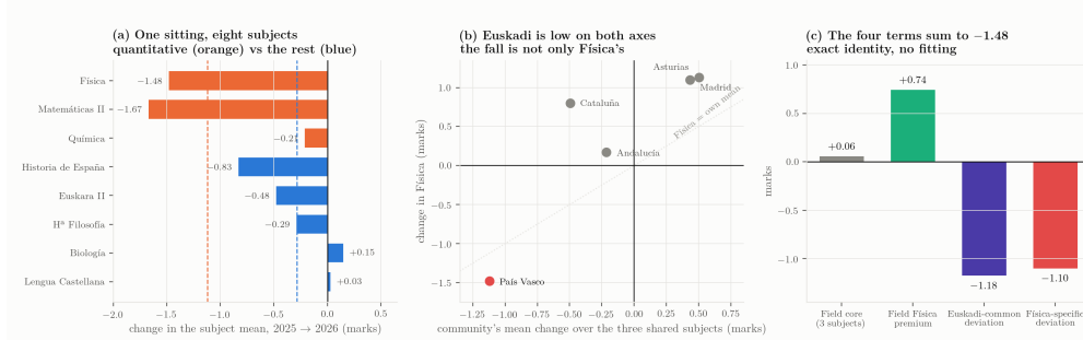
Figure 2: a — the eight Basque subjects, with the three the numerical marking deductions can reach in orange. b — each community's Física change against its own mean over the three shared subjects. c — the four terms of the split, which sum to the observed -1.48 by construction.
