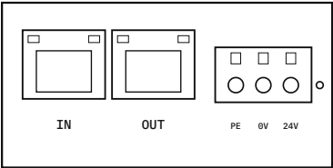
CK-EC5163 (TOP)
