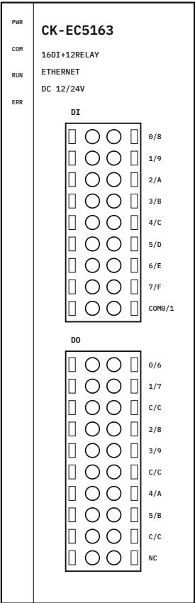
CK-EC5163 (FRONT)
