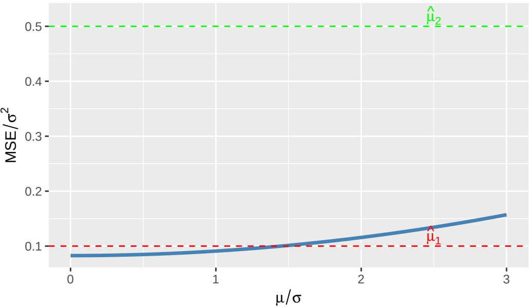
MSE Comparison ( n = 10 )
