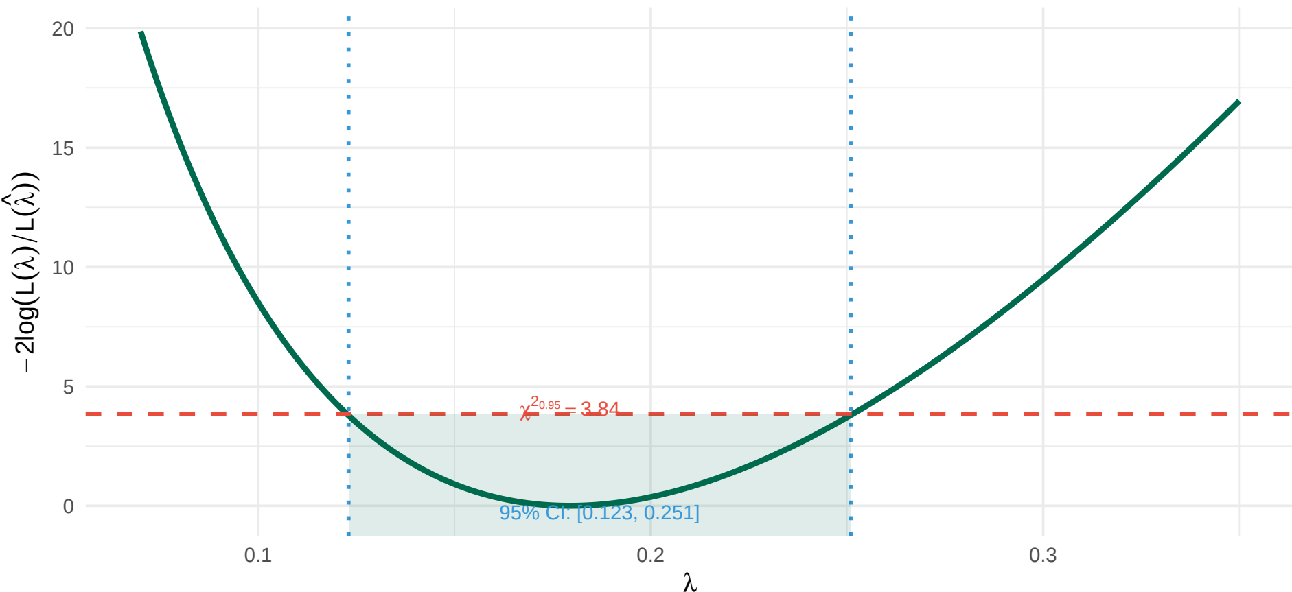
Profile Likelihood CI for LOS rate \lambda
