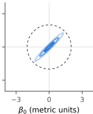
(b) rotated, diagonal corr +0.97, \kappa = 4,521
