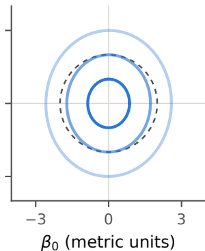
(c) rotated, dense block corr +0.01, \kappa = 368
