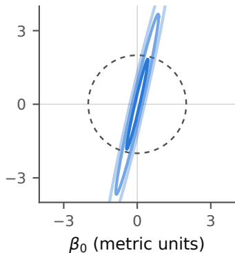
(a) unrotated, diagonal corr +0.97, \kappa = 5,555
