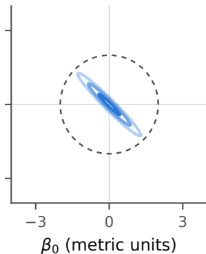
(b) rotated, diagonal corr -0.97, cond. 4,521
