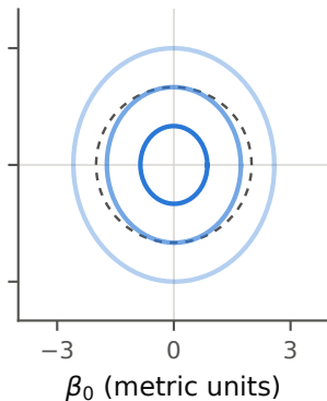
(c) rotated, dense block corr -0.01, cond. 368
