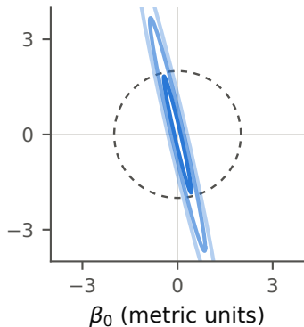
(a) unrotated, diagonal corr -0.97, cond. 5,555
