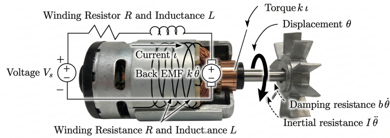
Figure 3: Electromechanical model of a DC motor. The electrical circuit represents the internal winding resistance ( R ) and inductance ( L ), while the mechanical side illustrates the conversion of current into torque to overcome rotor inertia and viscous damping.
