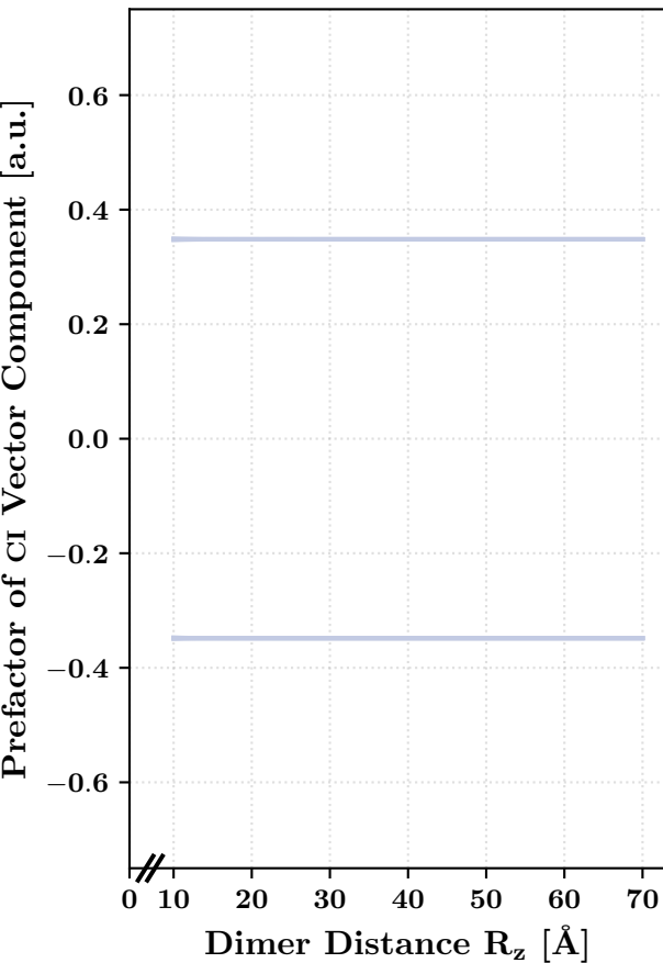
State 2.8
