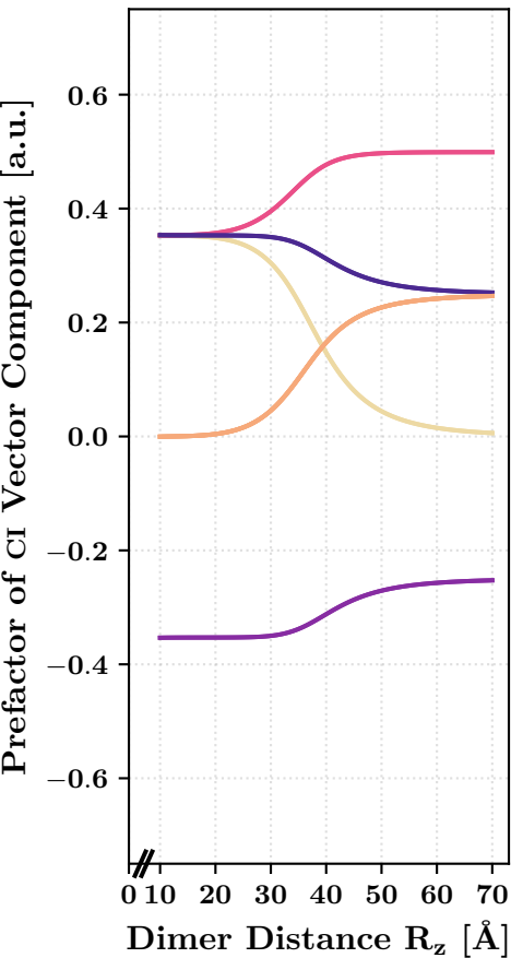
State 4.1
