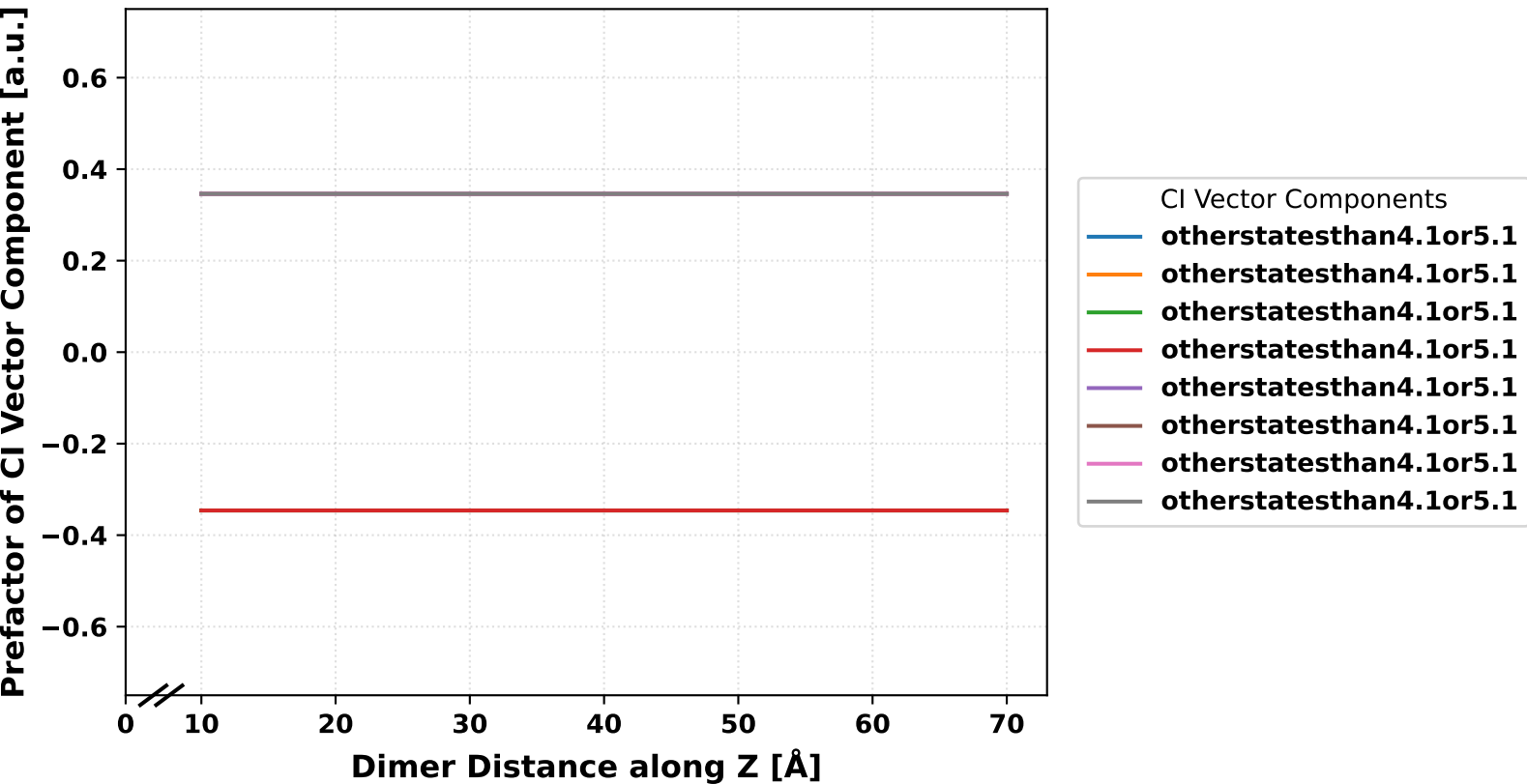
state 2.4
