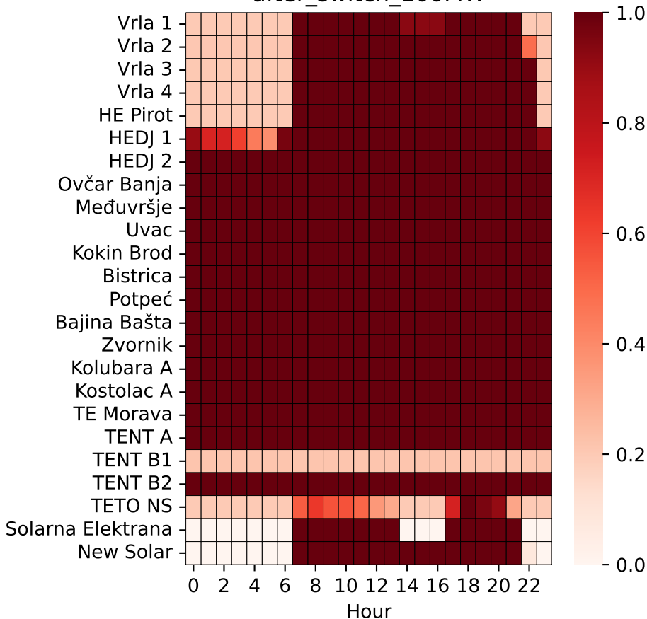
after_switch_100MW
