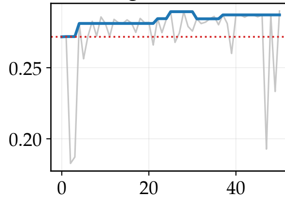
Avg nDCG@10
