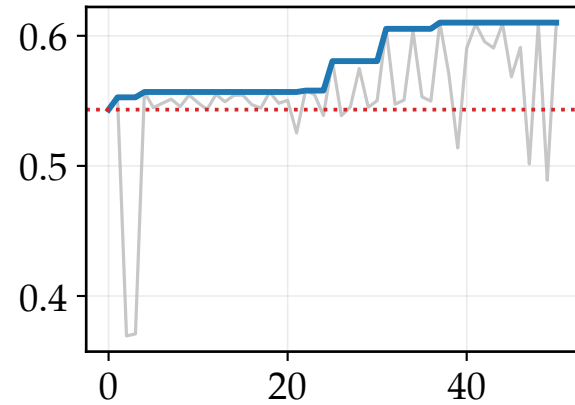
Combined score
