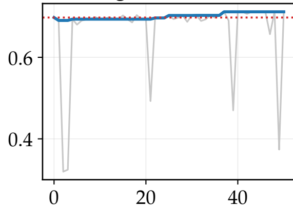
Avg Recall@1000
