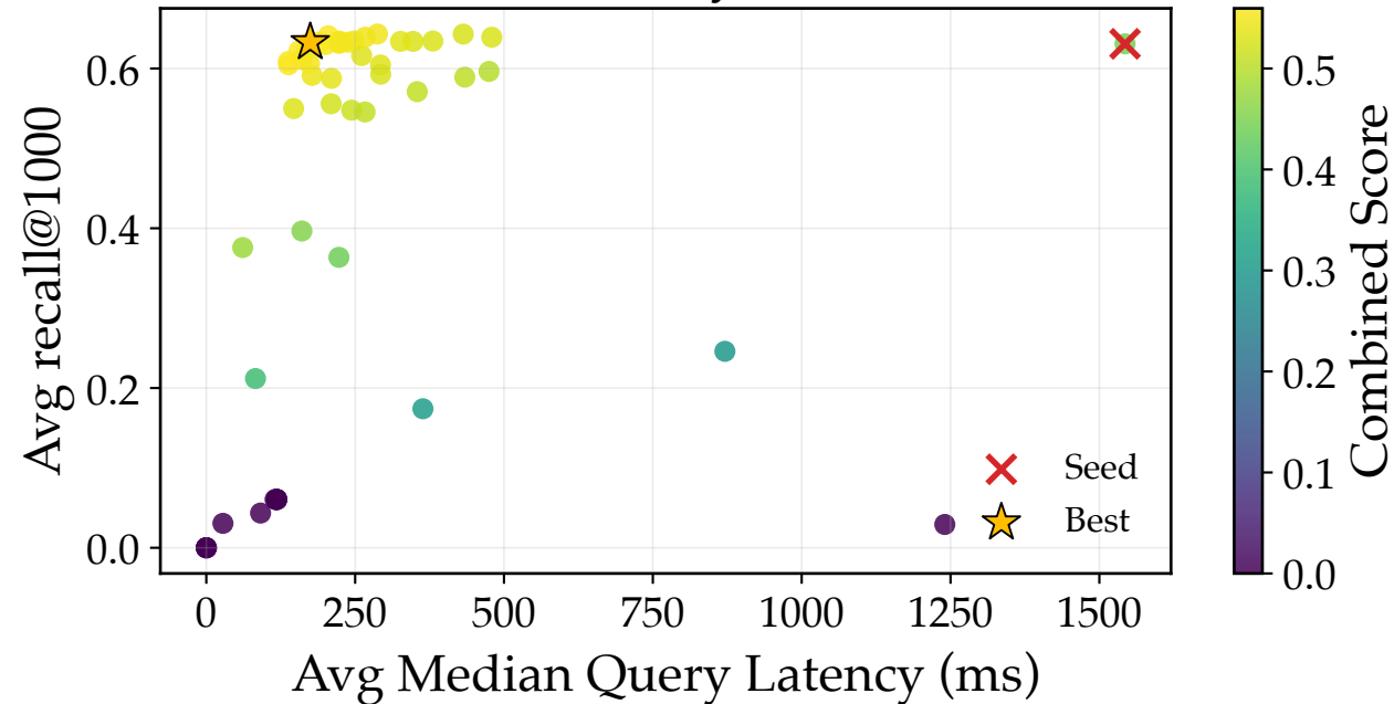
Recall / Latency Tradeoff
