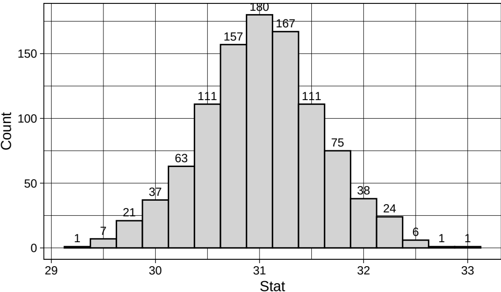
Histogram of 1000 simulated statistics under the null hypothesis
