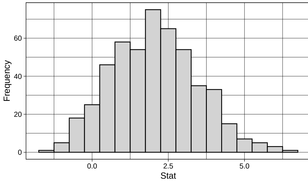
Histogram of 500 Simulations via Bootstrapping
