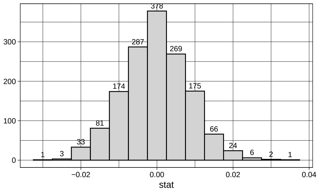
Histogram of 1500 Simulated statistics under the null hypotheses
