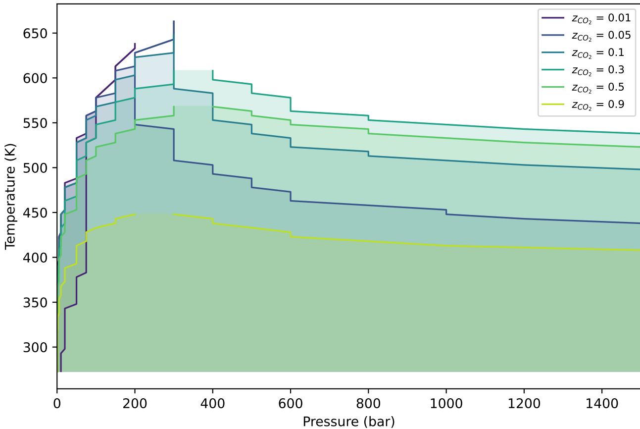
Two-Phase Envelope (CPA, CO 2 + H 2 O)
