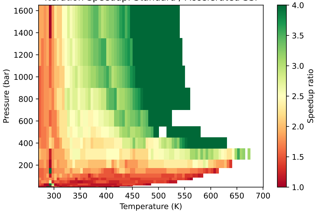
Iteration Speedup: Standard / Accelerated SSI
