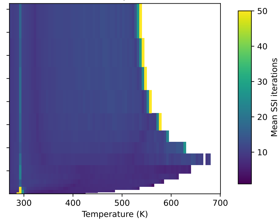
Accelerated SSI (Stability K)
