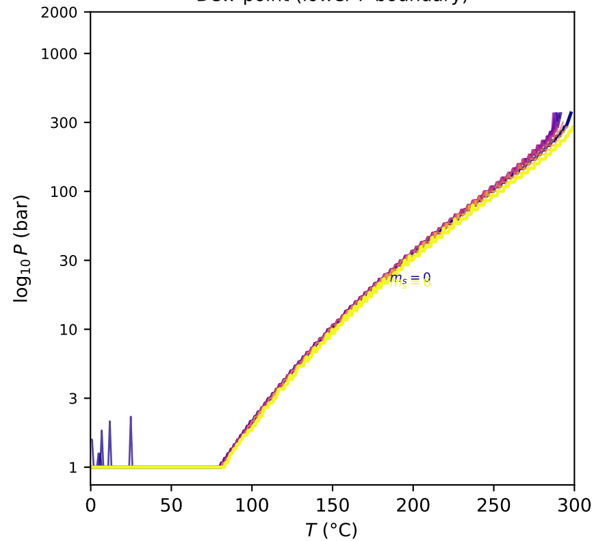
Dew-point (lower P boundary)
