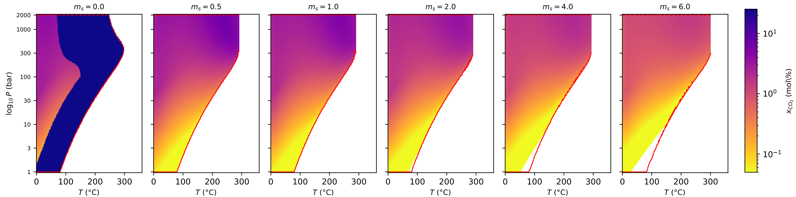
Equilibrium CO 2 mol\% in aqueous phase ( z = 0.5 )
