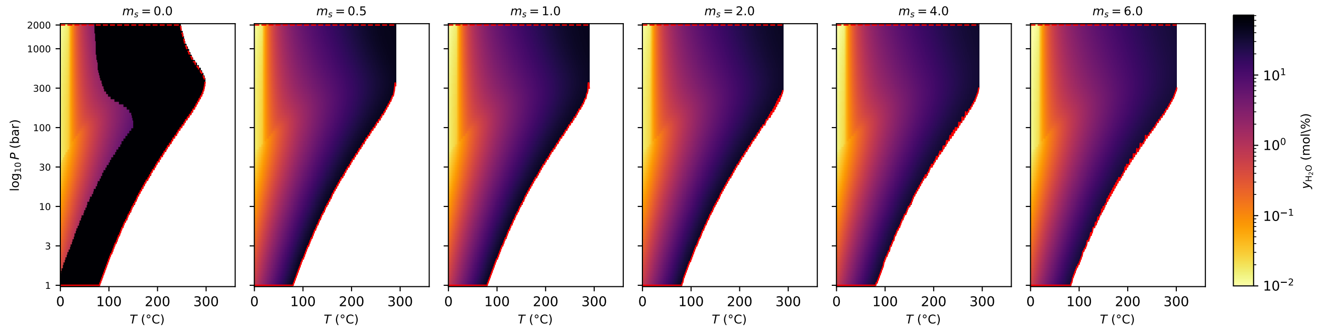
Equilibrium H 2 O mol\% in CO 2 -rich phase ( z = 0.5 )
