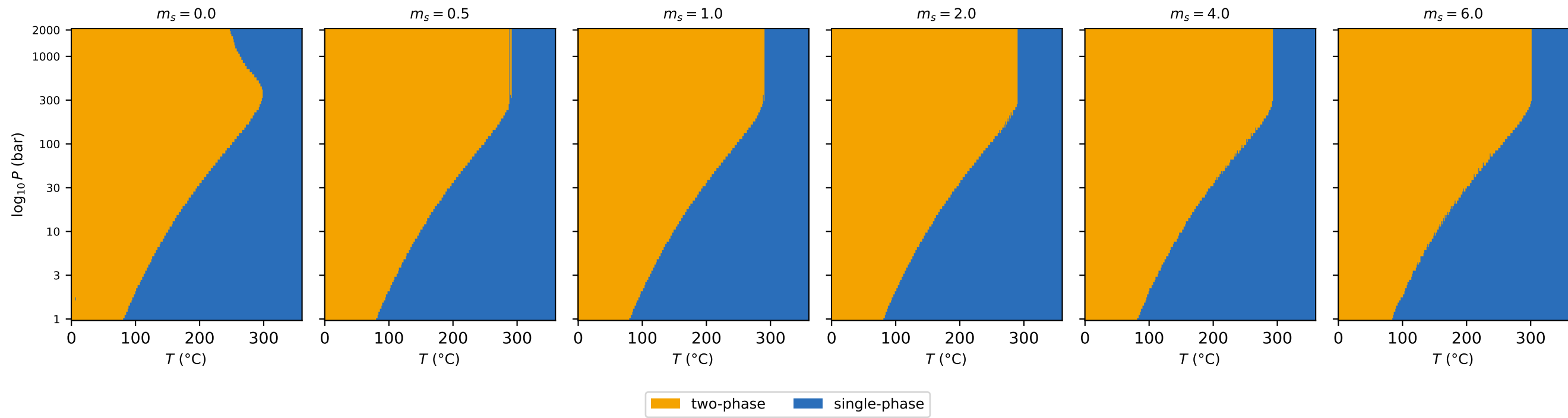
Phase state at representative feed z = 0.5
