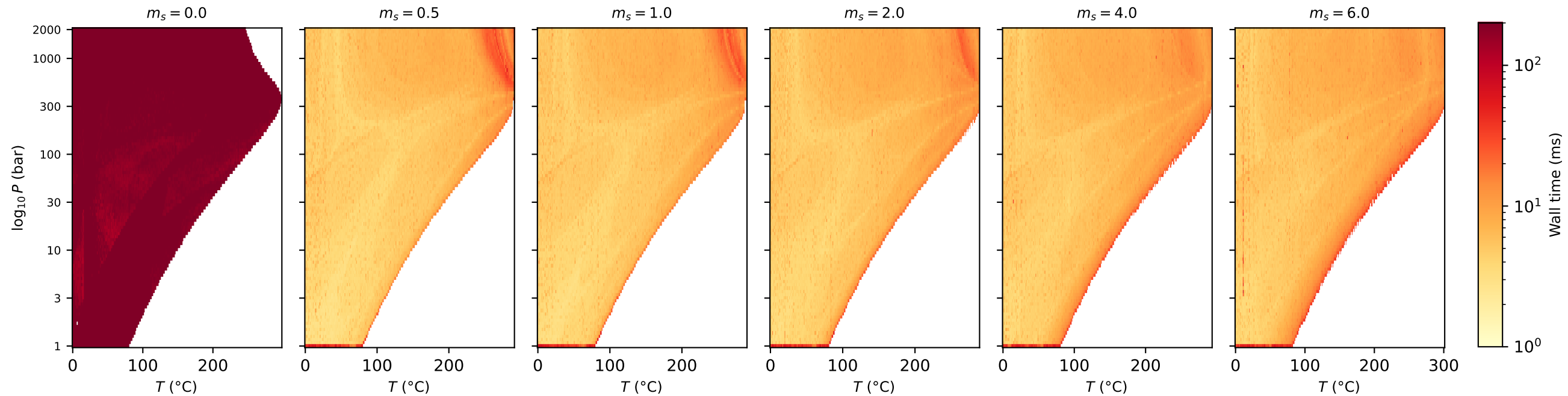
Mean wall time per flash call (ms), two-phase points only
