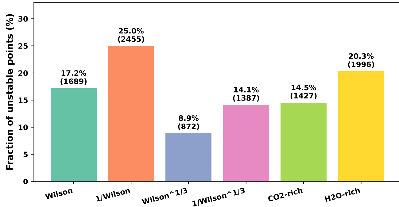
Best Stability Initial Guess (lowest TPD)
